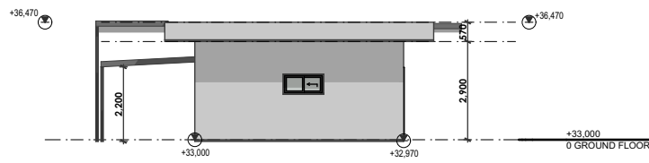
2 SOUTH ELEVATION 1:200
