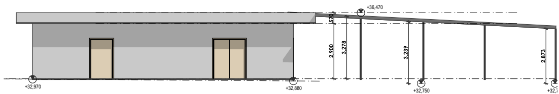
4 EAST ELEVATION 1:200
