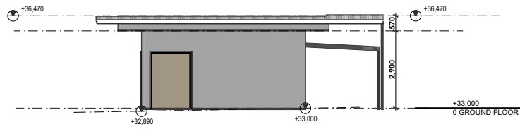
1 NORTH ELEVATION 1:200
